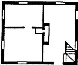
FIGURE 2.1 SAMPLE FLOORPLANS OF REPRESENTATIVE LANCASTER COUNTY FARMHOUSES AND BARNES
