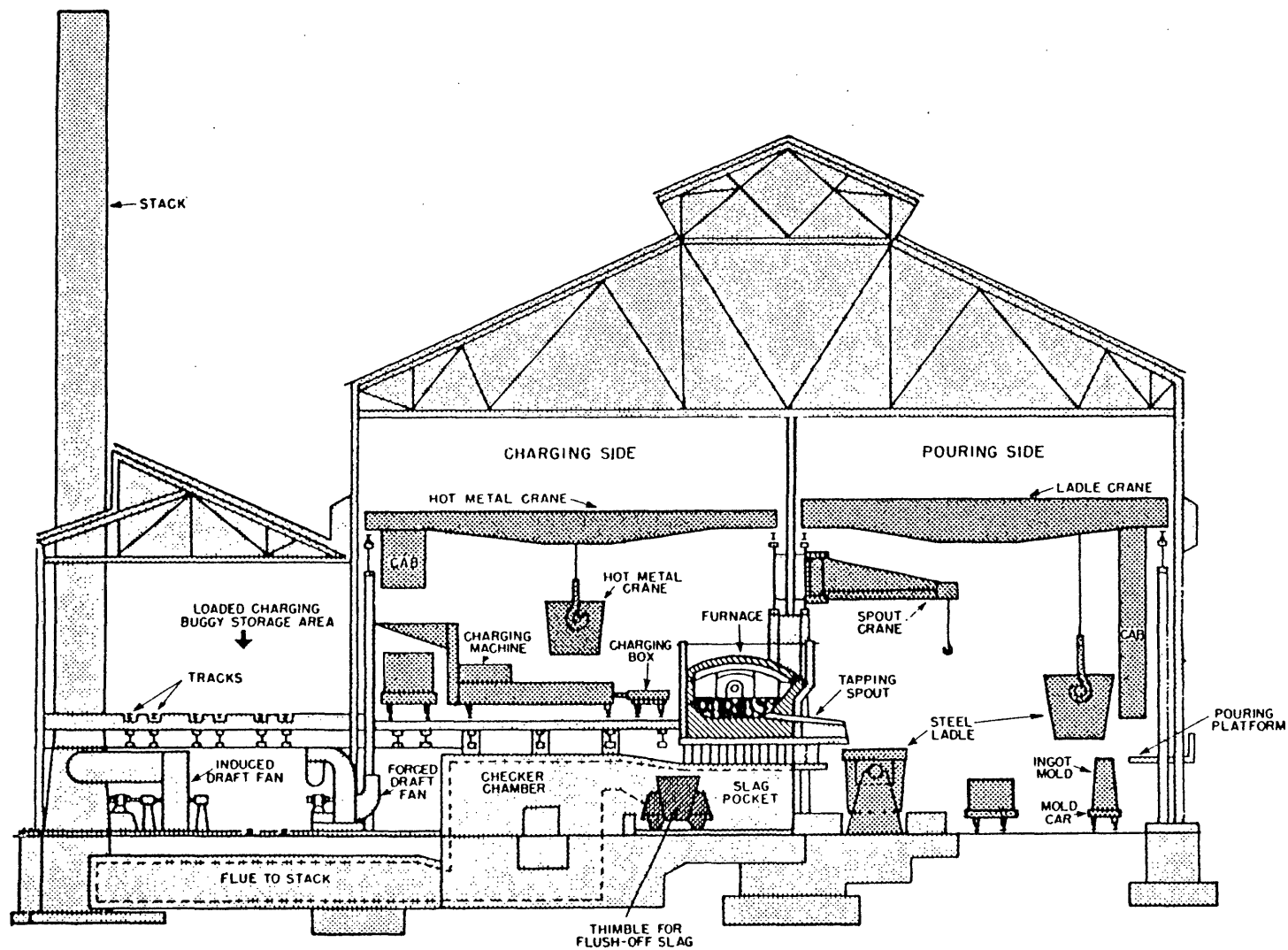
Cross section of an open hearth plant. The open hearth furnace is located in the middle, with charging floor, charging box, charging machine, and overhead travelling crane to the left. Further to the left is the stack and more loading storage space. To the right of the furnace is the pouring pit with overhead travelling crane, ingot mold, and ladles. A checker chamber and slag pocket are shown underneath the furnace. (Source: William T. Hogan, Economic History of the Iron and Steel Industry in the United States (Lexington, MA.: Lexington Books, 1971), 2: 407.)
