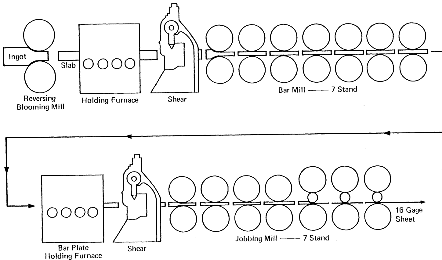
A schematic diagram of the Ashland Strip Mill. Later fully continuous strip mills eliminated the bar plate holding furnace so that steel was passed directly from the bar mill to the jobbing mill. (Source: William T. Hogan, Economic History of the Iron and Steel Industry in the United States (Lexington, MA.: Lexington Books, 1971), 3: 849.)
