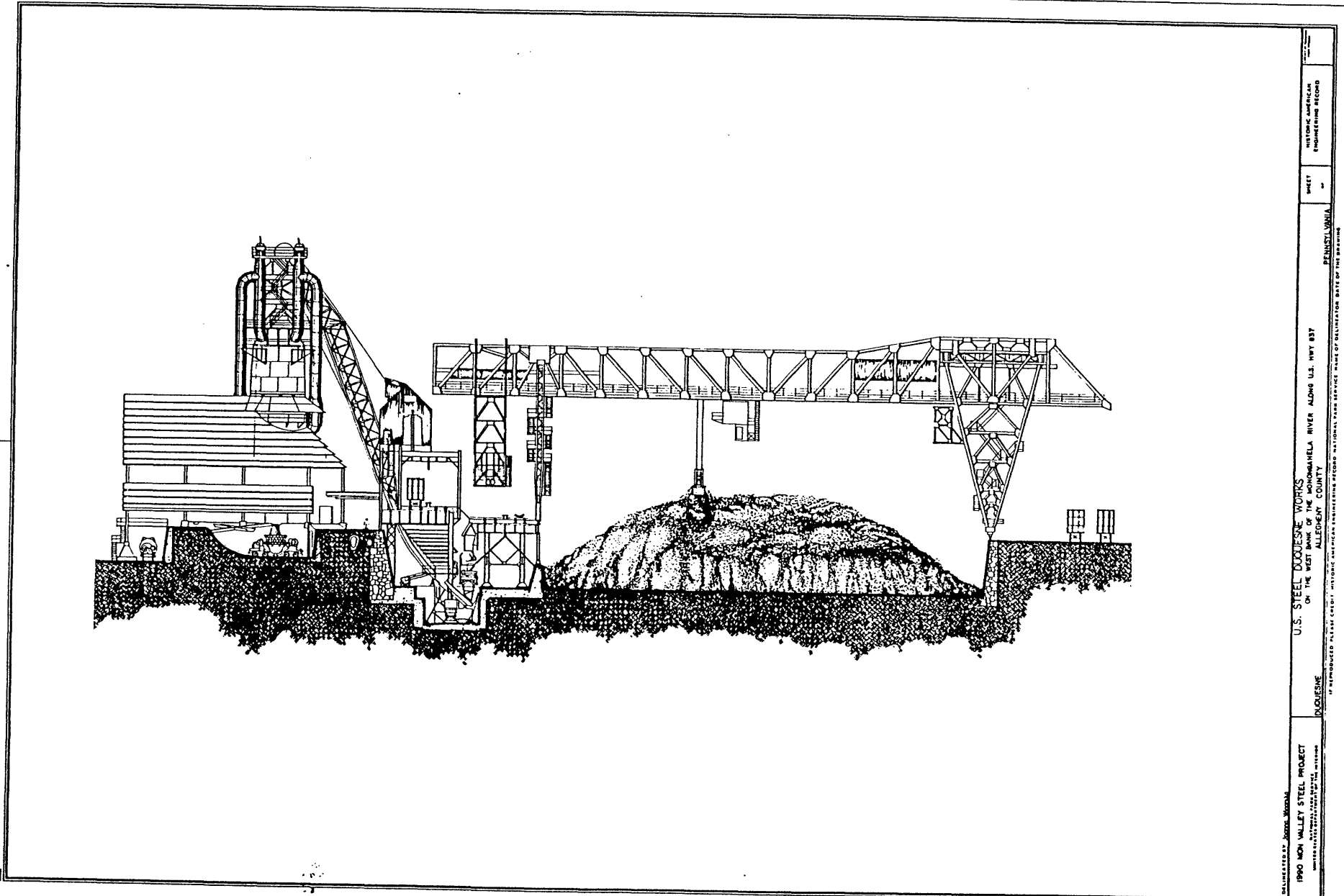
Duquesne Blast Furnace No. 1, as it appeared in 1990, with the ore bridge to the right, blast furnace to the left, and skip hoist and loading facilities in between. (Source: Historic American Engineering Record.)
