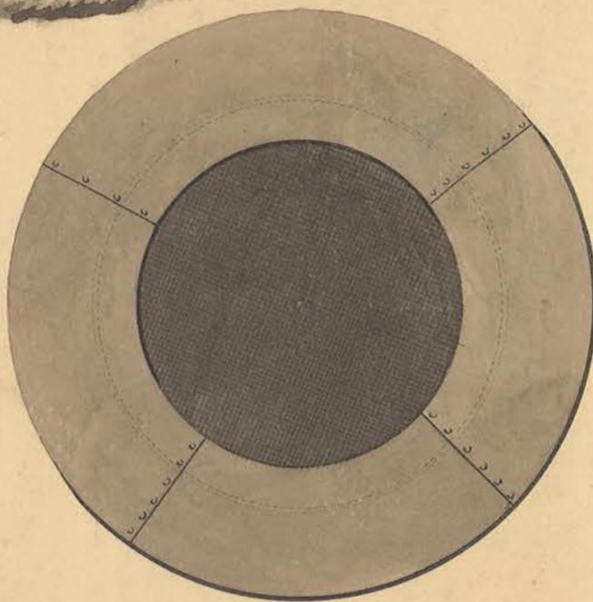
HORIZONTAL VIEW OF TOP OF CHIMNEY.
