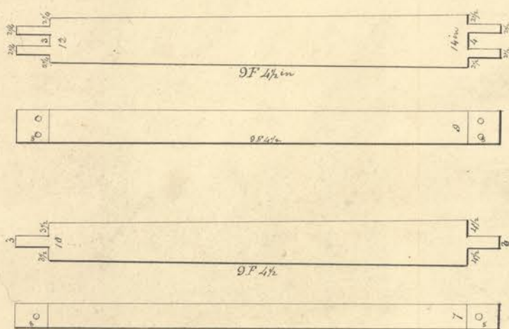
Ribs of Gates with their tenons Pins 1/4 in. Centre of hole 2 1/4 in from shoulder
