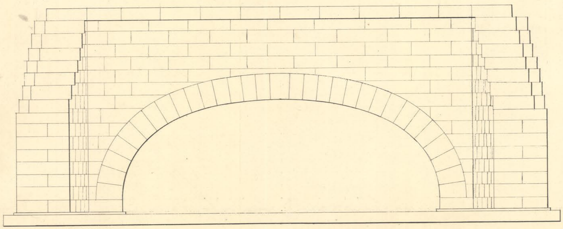
End View.
