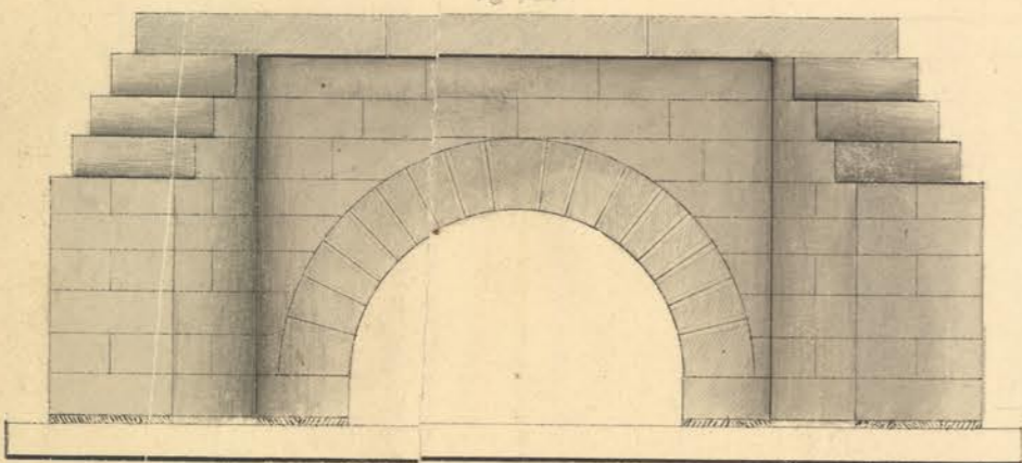
Section at End —
