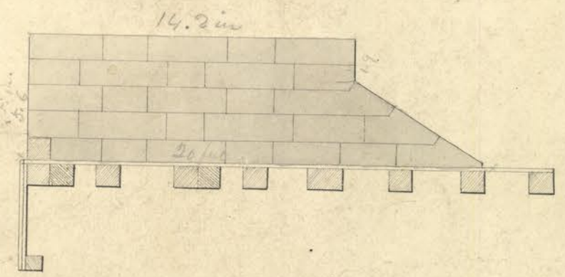
SECTION at Pier without frame
