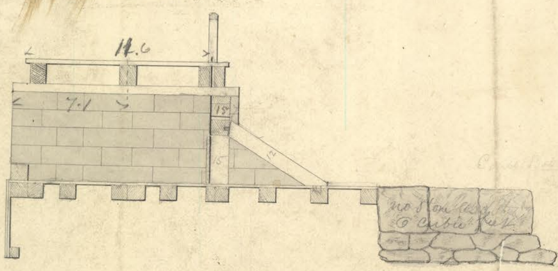
SECTION at Pier
