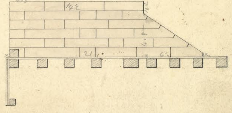
SECTION of Pier (without Frame).
