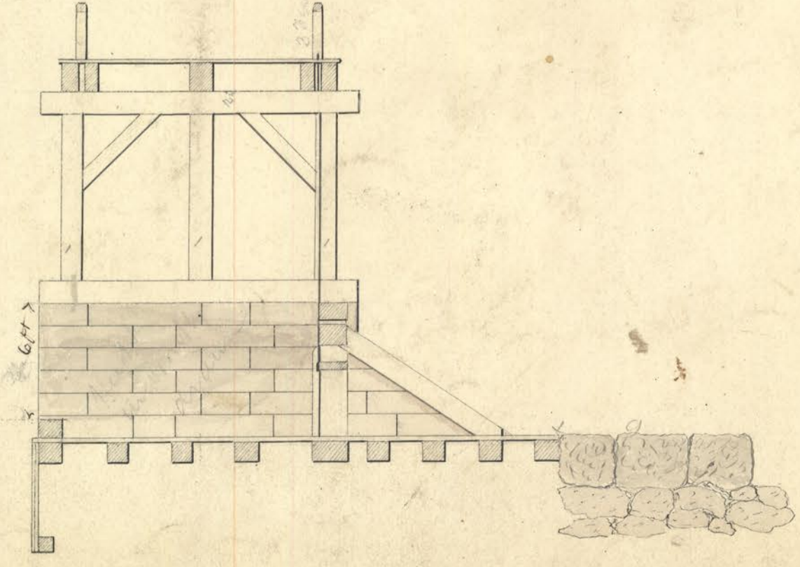
SECTION at Pier.
