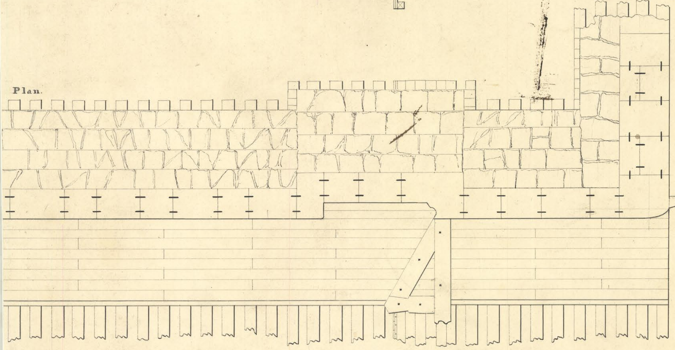
Section Centre of Lock.
