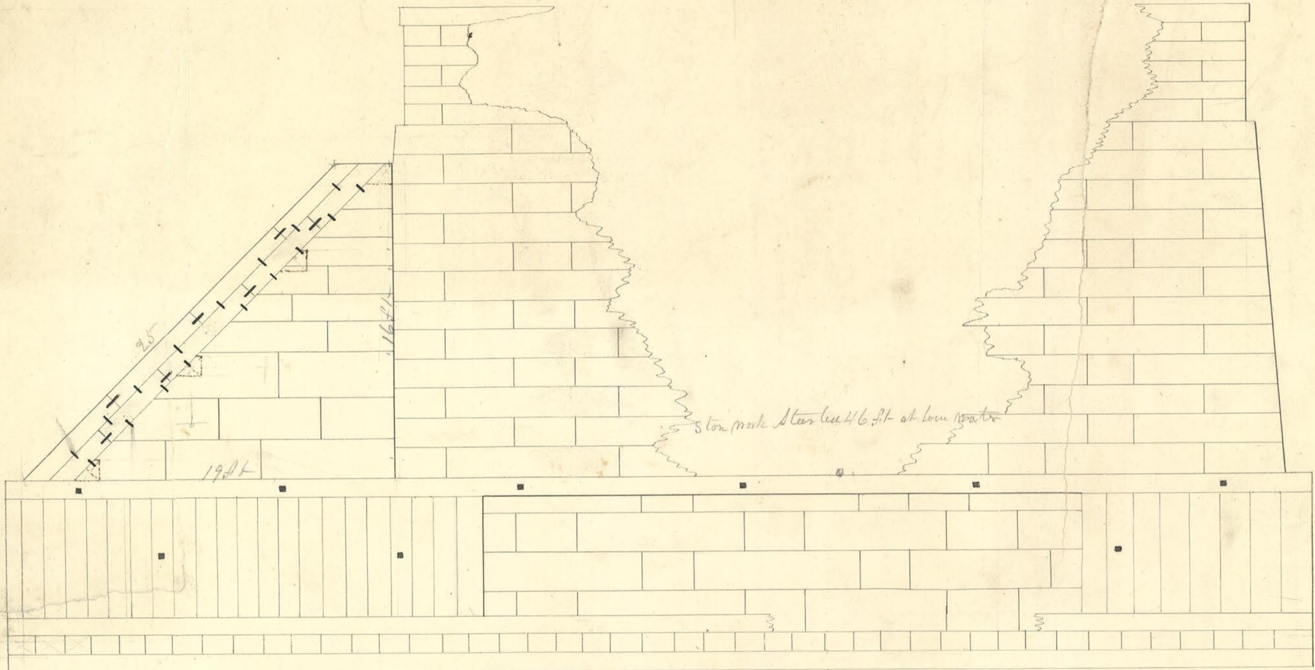
Section of Pier
