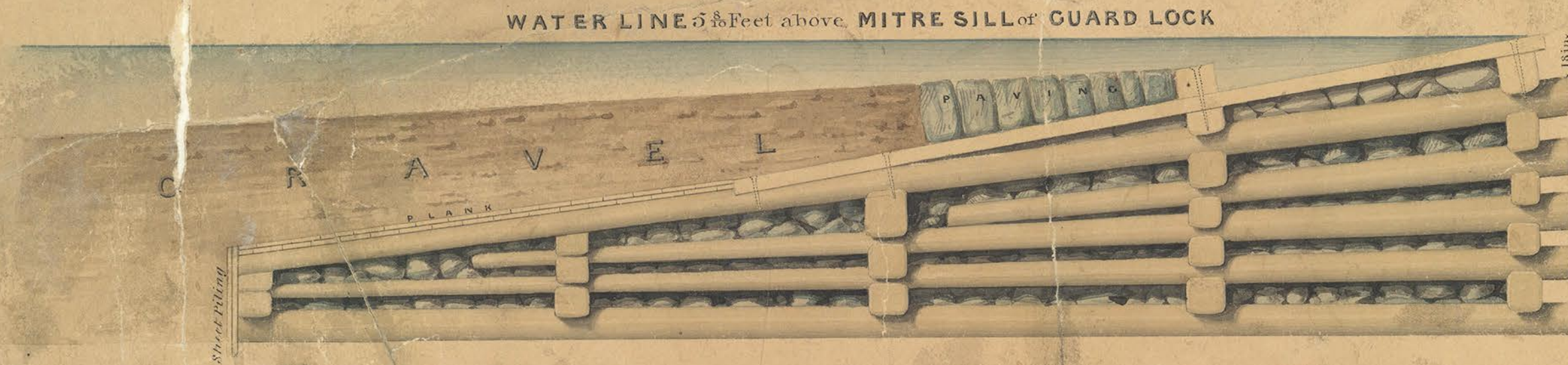
TRANSVERSE SECTION of the DAM near the WESTERN ABUTMENT Exhibiting the PLAN of the REPAIRS of 1840
