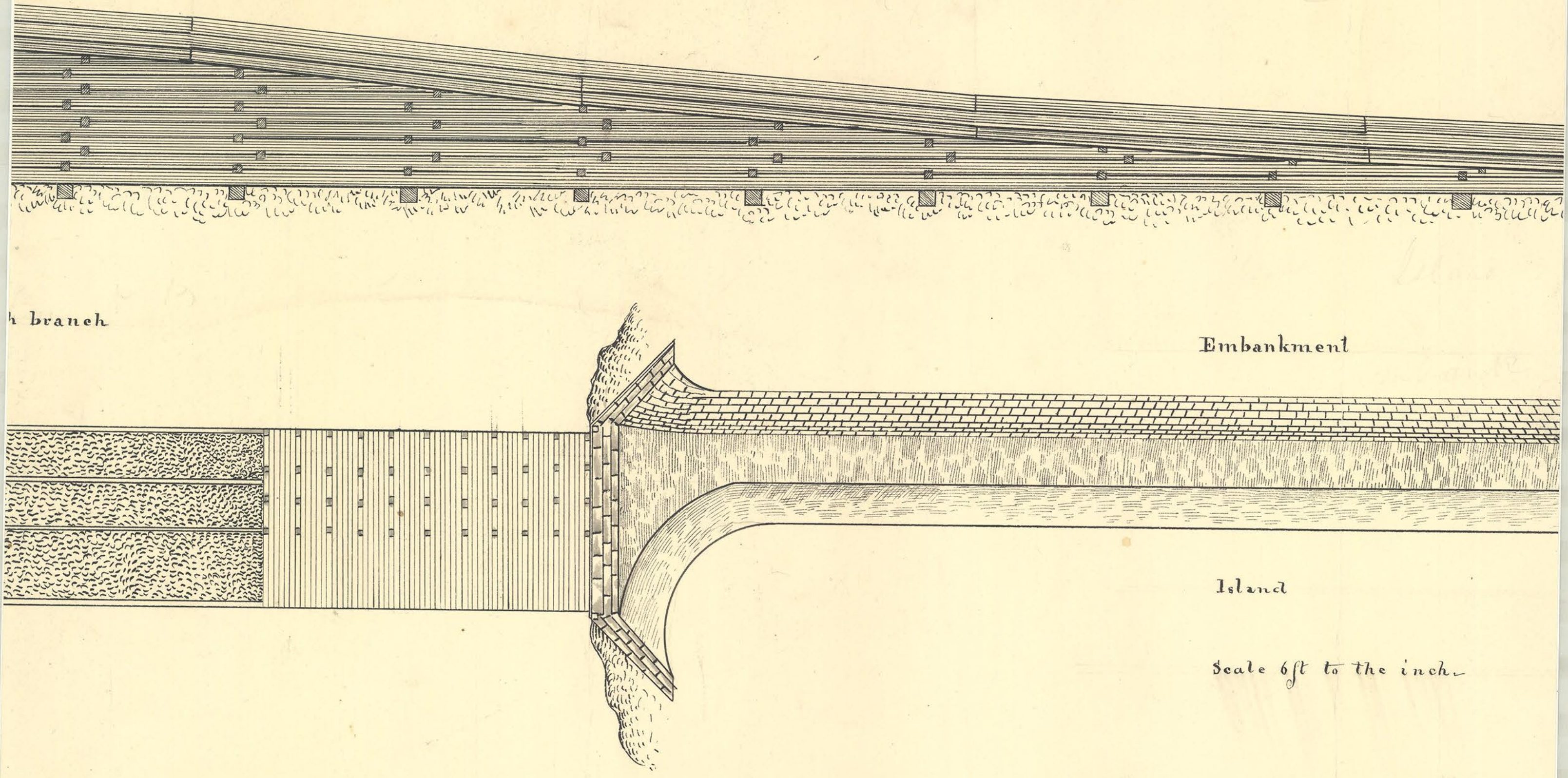
Elevation of Shute
