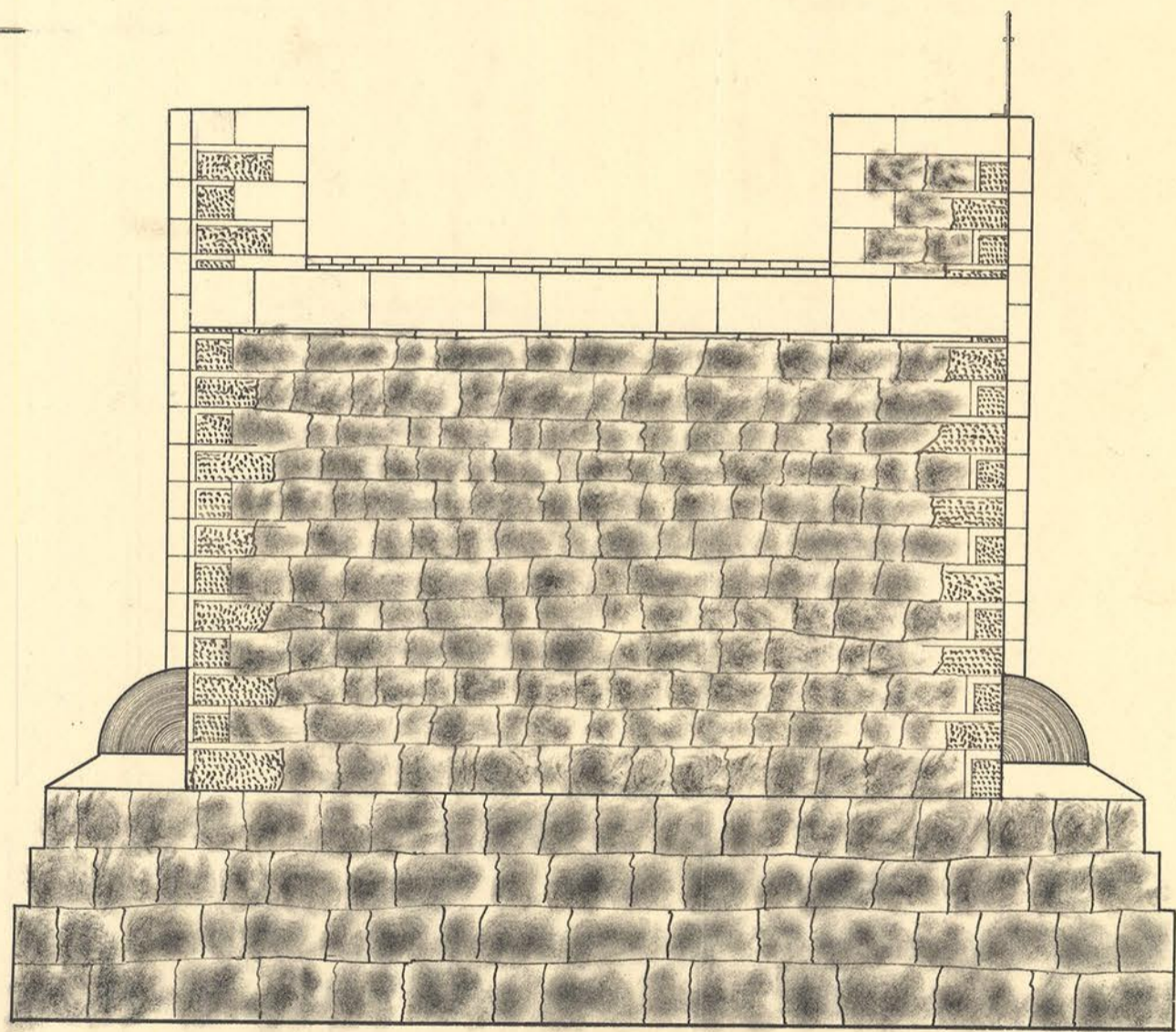
Cross Section
