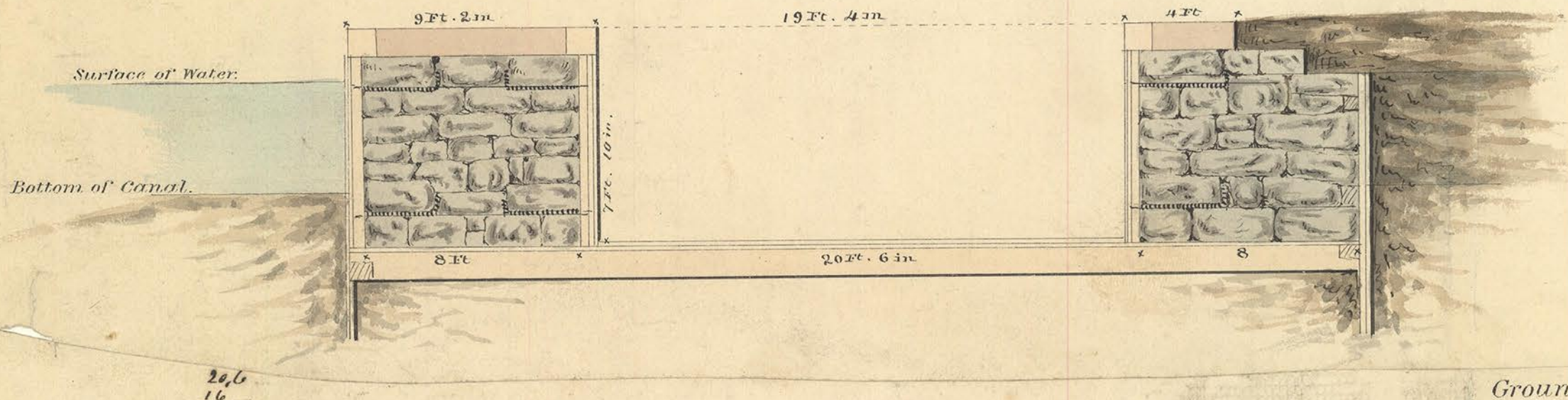
Cross Section in Recess for Cradle.
