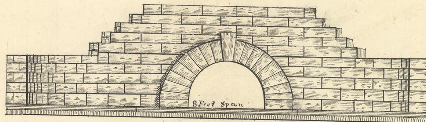
End View
