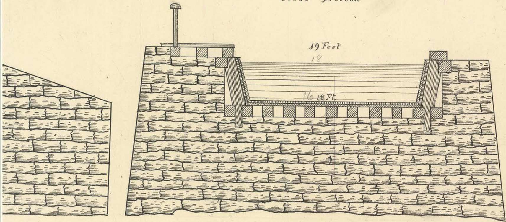
Cross Section
