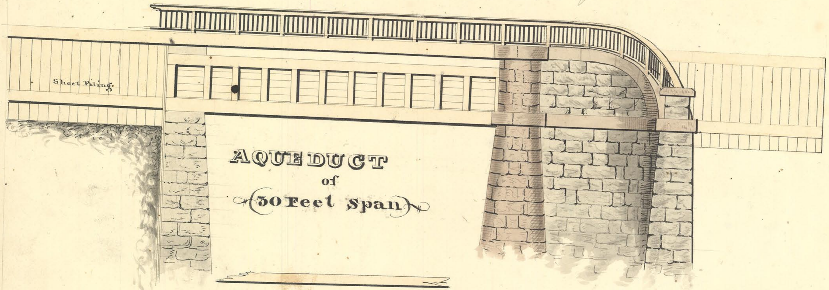
Plan for Aqueducts No. 1, 2 & 3
