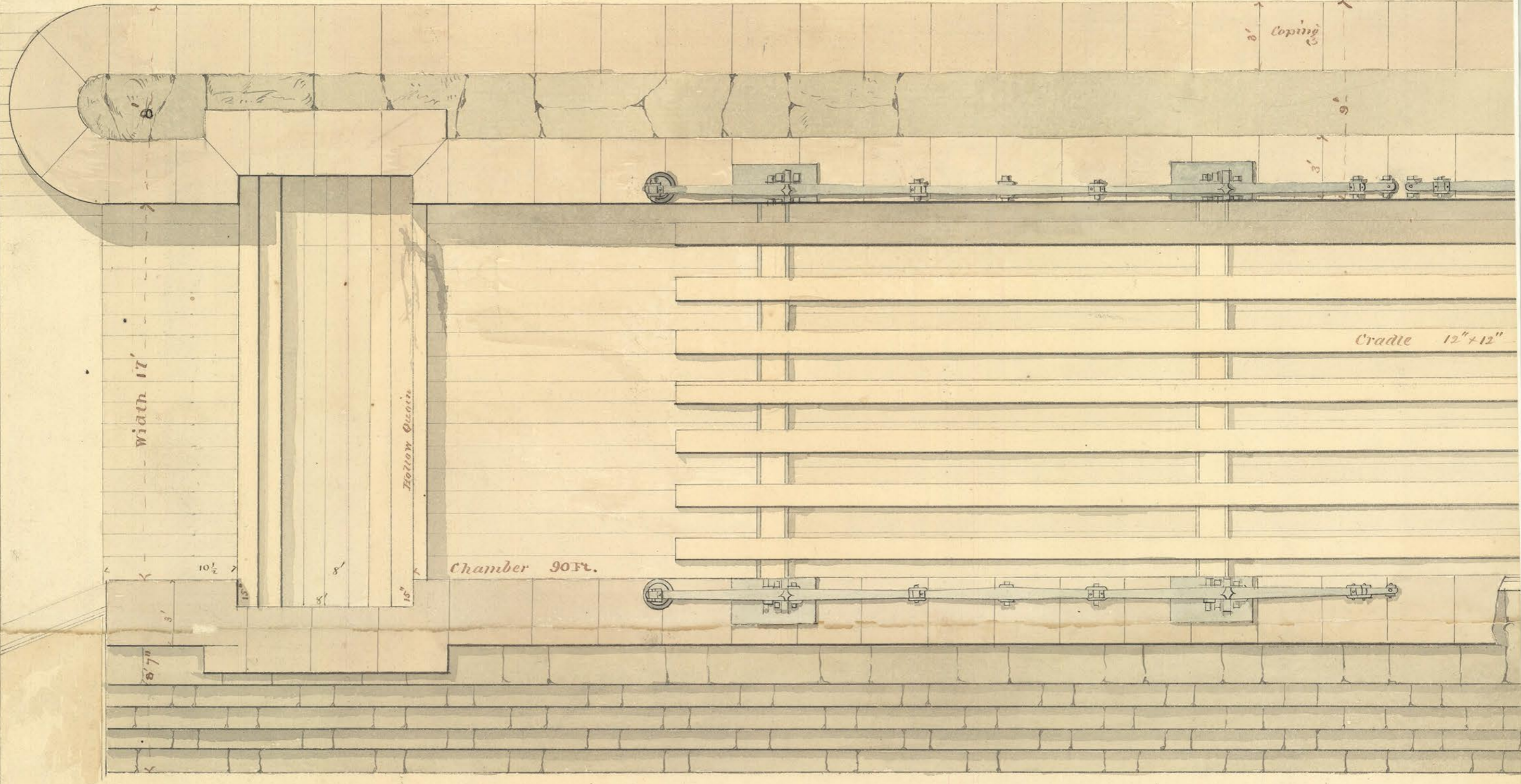
Sketch of Weigh Lock at Huntingdon. Scale 1/2 Ft. to an Inch.
